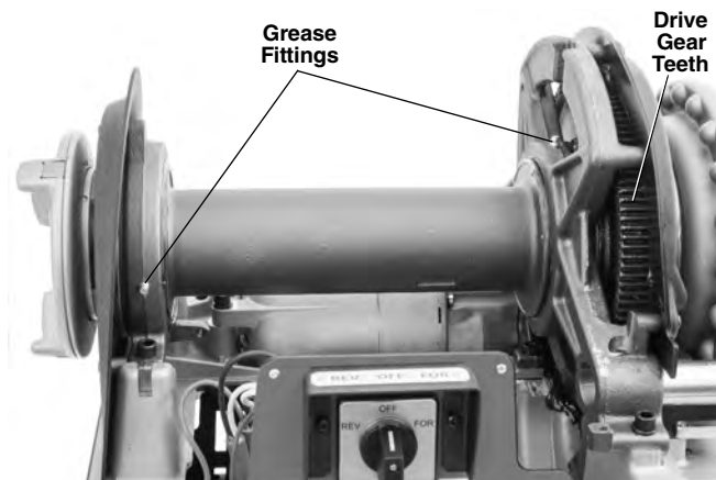
Figure 29 – Lubrication Points
