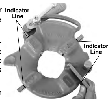
Figure 6 – Inserting Dies
