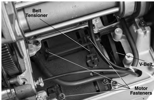
Figure 35 – Belt Tensioning
